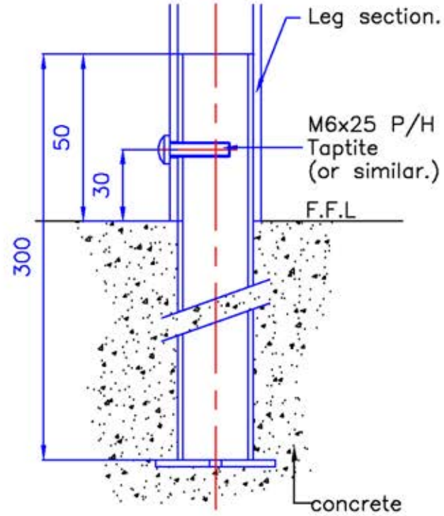
Built-in fixing method using optional 'C' spigot
